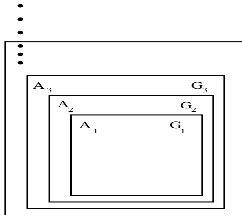
Figure 1: An incomplete formal system of mathematics.
