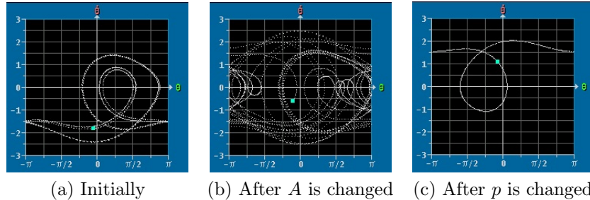
Figure 6: Phase plane diagrams before, during, and after sequential changes
