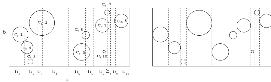
Fig. 4. Separating the coins horizontally with n moves.
