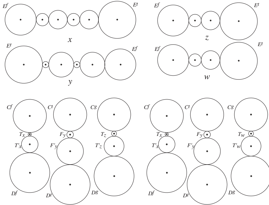
Fig. 9. A placement of coins that corresponds to the the 1-in-3SAT instance (x, y, z), (x, y, w) , and the truth assignment y = \mathbf{true} and x = z = w = \mathbf{false} . Note that this representation does not assign distinct sizes to the coins as specified by the construction. Using sizes as specified would require a drawing that is too big to be practical. We also have altered our notation in the figure to better suit the example. The intended meaning should be clear.
