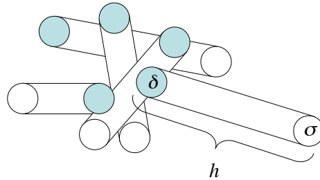
Fig. 5. The hippodromes corresponding to coin trajectories. The shaded discs represent destinations. We have labeled one hippodrome to illustrate the areas h , \sigma , and \delta .
