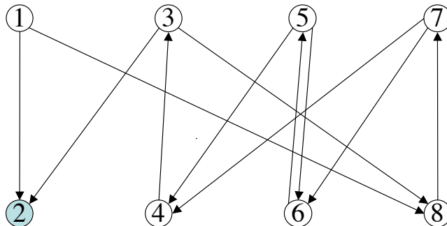
Fig. 6. There are coins at every position except 2. Observe that we can move the coins with an itinerary: 3 \rightarrow 2 , 4 \rightarrow 3 , 5 \rightarrow 4 , 6 \rightarrow 5 , 7 \rightarrow 6 , 8 \rightarrow 7 , and 1 \rightarrow 8 . This itinerary traces a Hamilton path from 1 to 2 in reverse.
