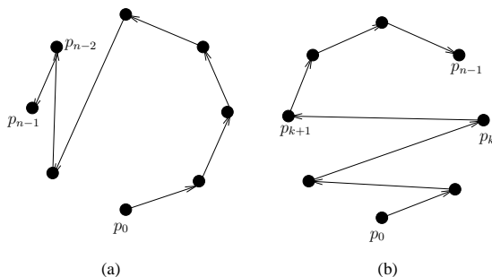
Figure 2: (a) Showing an example of case one with encoding [p_0, b_1, b_2, \dots, 0] (b) and case two with encoding [p_0, b_1, b_2, \dots, b_{k-1}, b_k, b_{k+1}, \dots, b_{n-2}] with b_k = 0 and b_t = 1 , for k + 1 \leq t < n - 1 .
