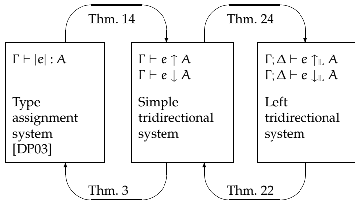
Figure 10: Connections between our type systems
