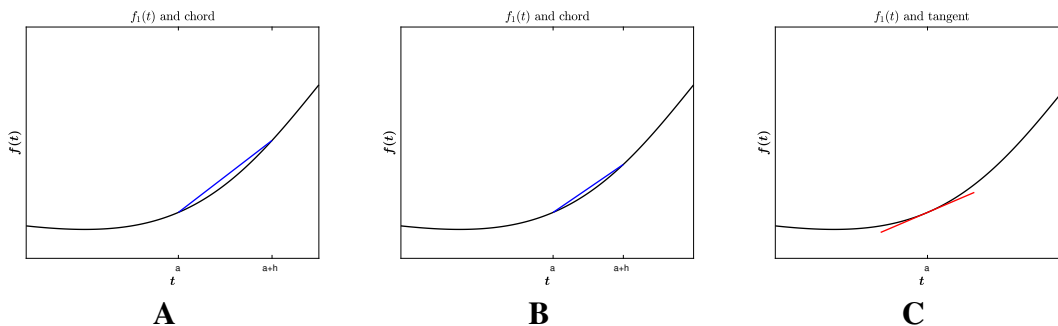
Figure 1: Graphically, the limit of a chord for f(t) between (a, f(a)) and (a + h, f(a + h)) is the derivative of f(t) at a . (A) A convex function f(t) , a scalar argument a , and a chord for a value h . (B) The same function and scalar argument, with a smaller value for h . (C) The derivative of f(t) at a is tangent to the curve of the function.
