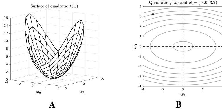
Figure 7.2: The function f_1(\vec{w}) in Equation 7.7. (A) Surface plot. (B) Contours and a point \vec{w}_0 .
