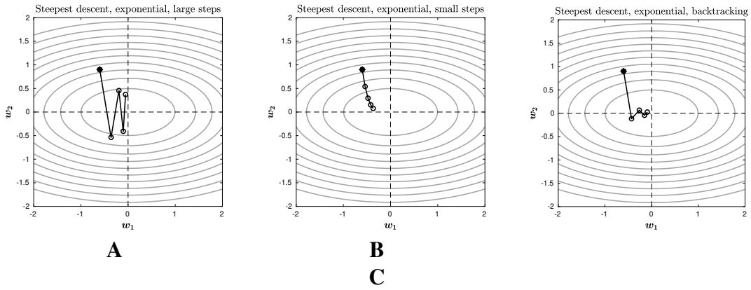
Figure 7.5: Steepest descent of the exponential function defined in Equation 7.8 using fixed and variable stepsizes. (A) Stepsize of s = 4 produces an oscillating path in the search space. (B) Stepsize of s = 1 converges slowly towards the minimizer. (C) Backtracking with s = 10 and \beta = 0.75 converges slower than quadratically selected stepsizes and slows substantially near the minimizer.
