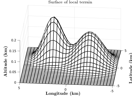
Figure 7.1: A function that represents local terrain. From any point, we might try to descend in the steepest direction to arrive at a river in a valley.
