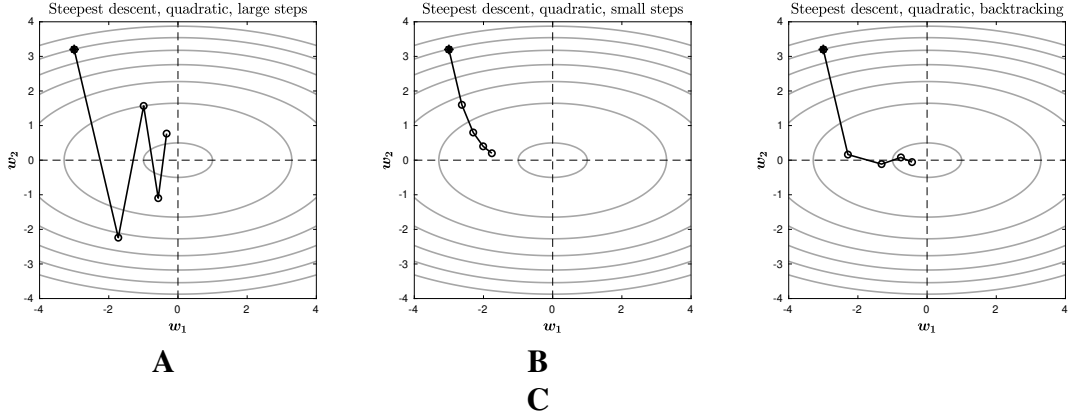
Figure 7.4: Steepest descent of the function defined in Equation 7.7 using fixed and optimal stepsizes. (A) Stepsize of s = 0.85 produces an oscillating path in the search space. (B) Stepsize of s = 0.25 converges slowly towards the minimizer. (C) Backtracking converges slower than optimal stepsizes and with a less “jagged” search path.
