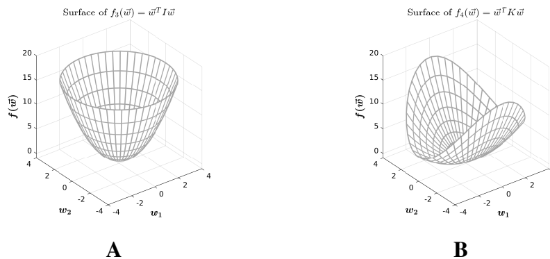
Figure 12.3: Quadratic functions, each with a 2D vector argument; these plot as paraboloids in 3D. (A) The function f_3(\vec{w}) defined in Equation 12.5 is a surface of revolution. (B) The function f_4(\vec{w}) defined in Equation 12.6 is not symmetric about the vertical axis.
