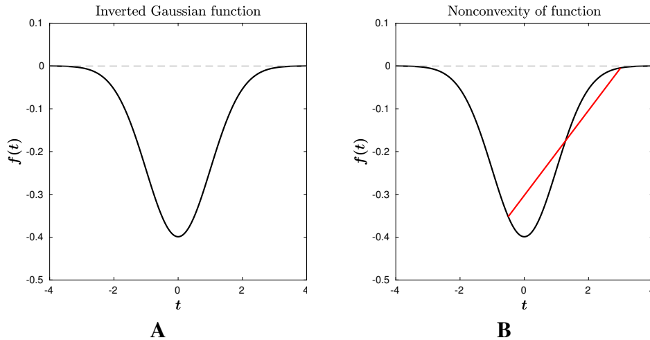
Figure 12.1: An inverted Gaussian is a function that monotonically decreases towards a minimum and that is not convex. (A) The function f(t) in Equation 12.1. (B) A chord between two points that intersects the graph of the function.
