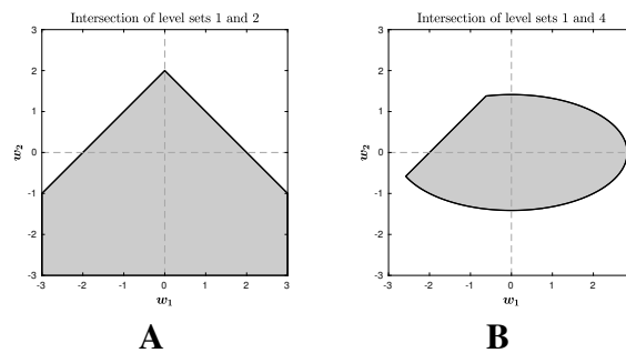
Figure 12.7: Level sets of convex functions that have a 2D vector argument, shown as shaded regions. (A) The intersection of the level sets \mathbb{S}_L(f_1, 0) and \mathbb{S}_L(f_2, 0) is a convex set. (B) The intersection of the level sets of \mathbb{S}_L(f_1, 0) and \mathbb{S}_L(f_4, 2) is a convex set.
