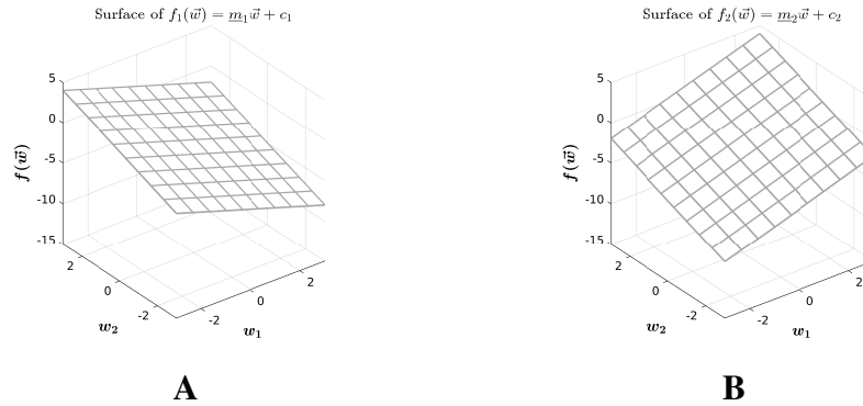
Figure 12.2: Affine functions, each with a 2D vector argument; these plot as planes in 3D. (A) The function f_1(\vec{w}) defined in Equation 12.3. (B) The function f_2(\vec{w}) defined in Equation 12.3.
