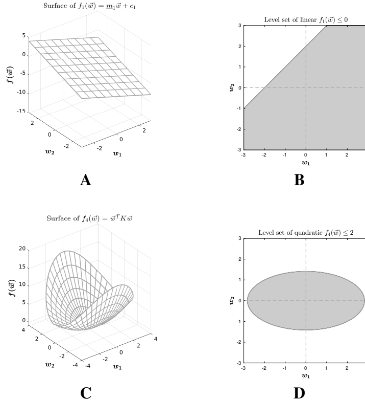
Figure 12.6: Surface plots and level sets of convex functions that have a 2D vector argument. (A) A surface plot of function f_1(\vec{w}) defined in Equation 12.3. (B) The level set of f_1(\vec{w}) \leq 0 , written as \mathbb{S}_L(f_1, 0) , is shown as the shaded region; the blue arrow is the direction of the transpose of the gradient of the function. (C) A surface plot of function f_4(\vec{w}) defined in Equation 12.6. (D) The level set of f_4(\vec{w}) \leq 2 , written as \mathbb{S}_L(f_2, 2) , is shown as the shaded region.
