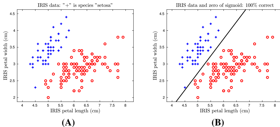
Figure 14.2: Vector representation of petal sizes for Fisher's iris data. Vectors for species Iris setosa are shown as blue crosses and vectors for other species are shown as red circles. (A) The data, labeled as in Fisher's article. (B) Classifications by a single sigmoidal artificial neuron; the 0-level contour of the sigmoidal function is shown as a black line.
