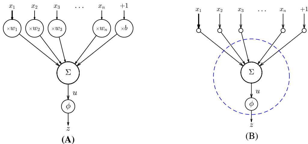
Figure 14.1: Illustrations of an artificial neuron. The input vector \vec{x} is scaled by the weights w_1, w_2, \dots, w_n and biased by b ; the result u is the input to the activation function \phi that produces the neuron output z . (A) Data flow for an artificial neuron. (B) The external parameter is the input \vec{x} and the output is z .
