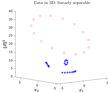
Figure 33.2: Pictorial data in 3D. The vectors with label +1 are plotted as a plus sign; vectors with label -1 are plotted as open circles.
